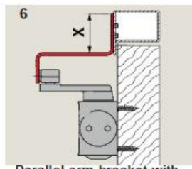
6 Parallel arm bracket with upstand
