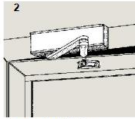
2 Frame installation
